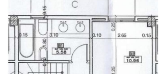
Dimensions and surfaces of the fifth floor
